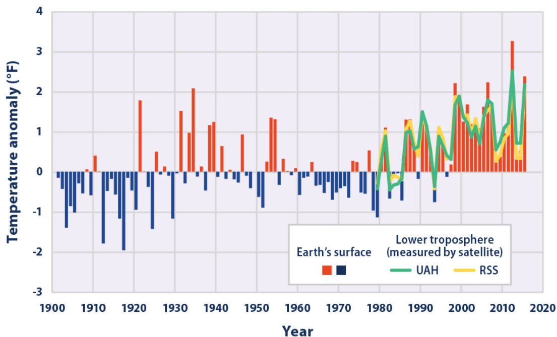
Figure 9. Temperature Anomalies
